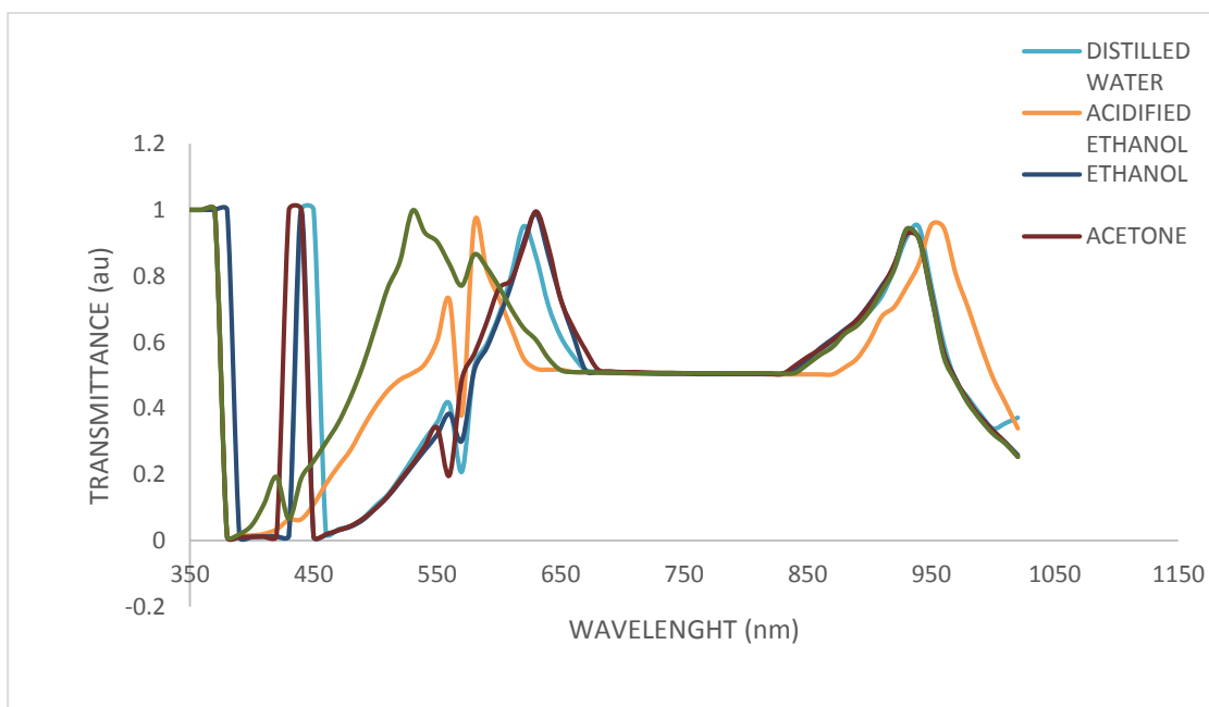
Figure. 4: Bougainvillea Transmittance Graph with Different Solvent.
